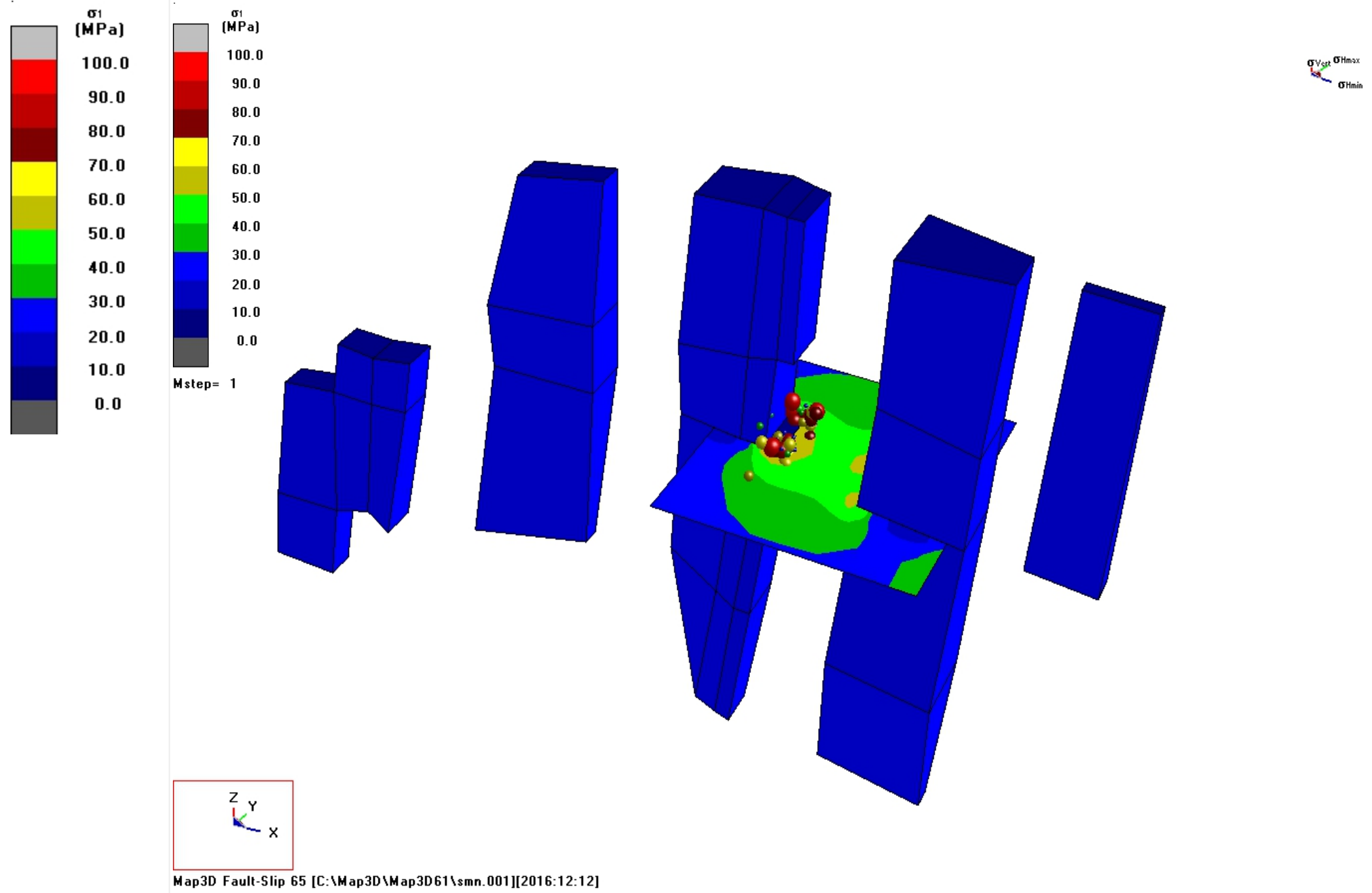
Seismic events superimposed on major principal stress contours.
